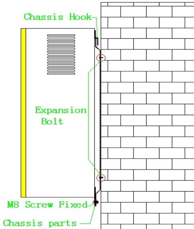
② Wall hanging installation diagram
